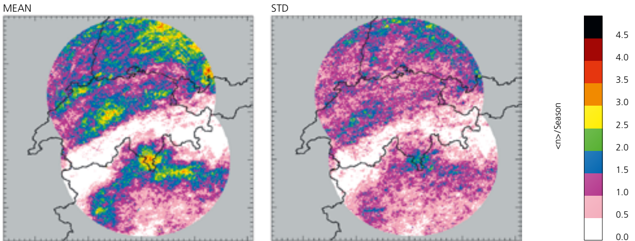
Left: average number of days with probability of hail > 80 % per season (April–September) and km 2 during the period 2002–2014; right: standard deviation of the number of radar-derived hail days per season. From Nisi et al. (2016).
