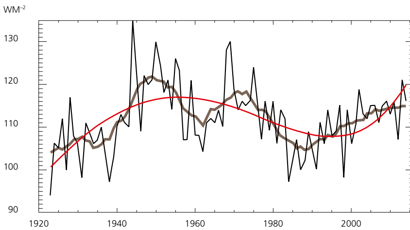
The longest continuous record available in GEBA: surface downward shortwave radiation ( Wm^2 ) measured in Stockholm since 1922. The brown line shows the 5-year moving average; the red line shows the fourth-order polynomial fit. Substantial multidecadal variations become evident, with an increase up to the 1950s (early brightening), an overall decline from the 1950s to the 1980s (dimming), and a recovery thereafter (brightening). (Adapted from Wild et al. 2017)
