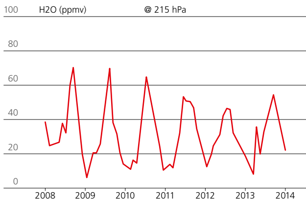
Time series of monthly mean water vapor volume mixing ratio at 215 hPa (approximately 11 km) measured by the Raman lidar at the regional center of Payerne. Only nighttime measurements taken under cloud-free conditions are considered. A distinct annual cycle is visible with a more humid tropopause region in summer.
