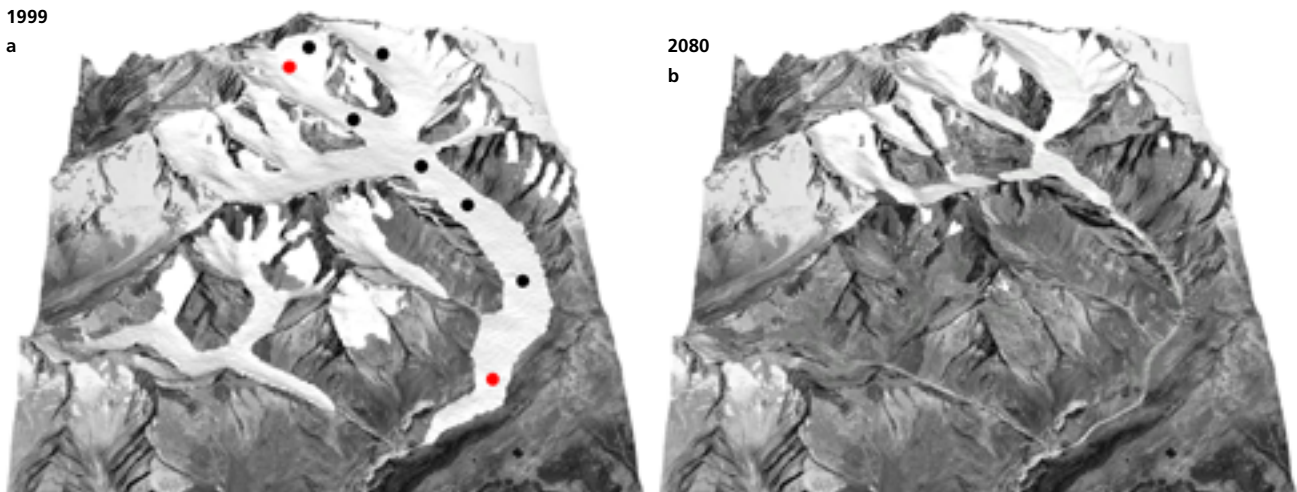
Modelled evolution of Grosser Aletschgletscher between 1999 and 2080 using a combined model for surface mass balance and ice dynamics. Long-term monitoring at individual sites (red dots: current measurement sites, black dots: historic sites) and combination of various data types is crucial for permitting projections into the future (figure adapted from Jouvet et al. 2011).
