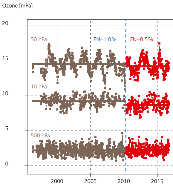
Ozone concentration time series at three characteristic levels in Nairobi, Kenya. The brown and red points display a change in the measurement procedures.
