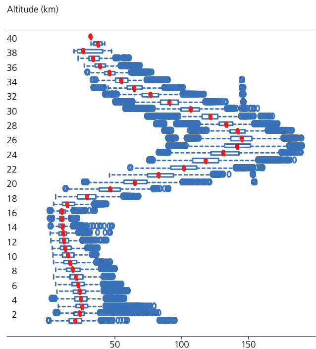
The IQR at all altitudes remains within ~20 nbar indicating a relatively small seasonal cycle at all altitudes.
