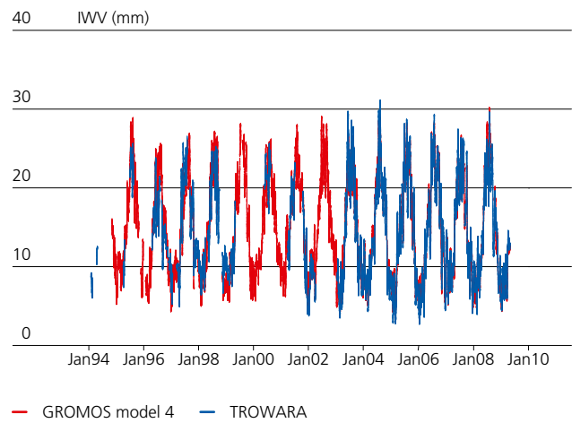
16-year time series of integrated water vapor above Bern measured by two microwave radiometers. Figure from Hocke et al., 2011.
