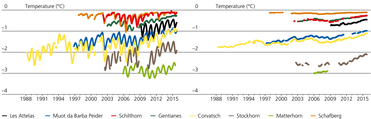
Ground temperatures measured in selected PERMOS boreholes. The data measured by the thermistors closest to 10 m (left) and 20 m (right) depth is plotted for each borehole. The exact depth is given in brackets in the caption.
