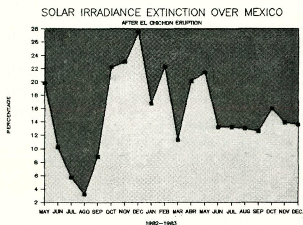
Figure 7.3: Monthly maximum solar radiance extinction over Mexico under cloudless conditions due to El Chichon stratospheric aerosol layer. From May 1982 to December 1983 (Galindo, 1992).
