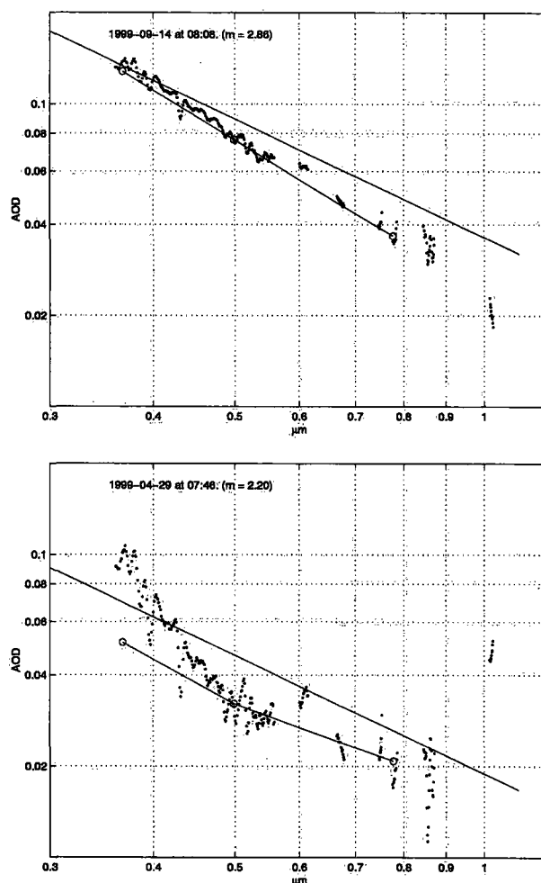
Figure 6.3: Examples of spectral AOD derived from measurements with LI-1800 ( \bullet ), CSEM2016 ( \circ ), and NIP (—).
