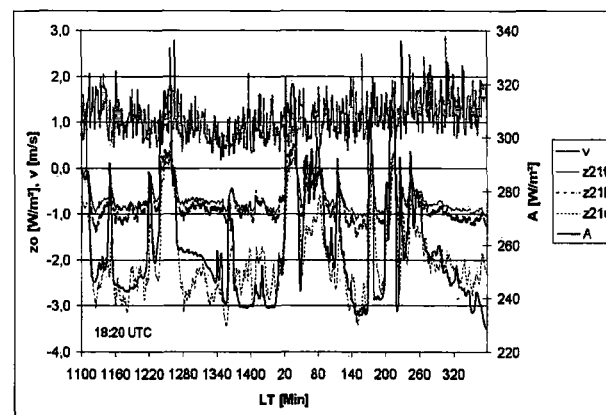
Figure 5.3: Night-time zero offset of three different ventilated CM21 (z21f: full power; z21h: half power; z21u: unventilated) and long-wave downward radiation A together with natural wind speed v Potsdam, 00-03-03/04
