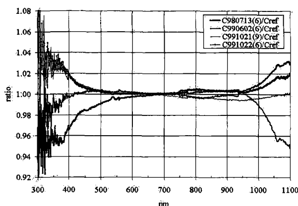
Figure 6.1: Lamp calibrations of LI-1800. Ratios of individual calibration results (spectral calibration factors) to the average of the results (Cref). Lamps: SP-6 and SP-9.
