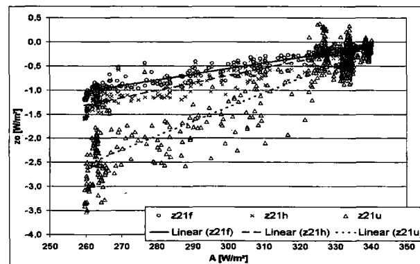
Figure 5.2: Scatter plot of the night-time zero offset of different ventilated CM21 (z21f: full power; z21h: half power; z21u: unventilated) and the corresponding linear regression lines in dependence on long-wave downward radiation A Potsdam, 00-03-06/07
